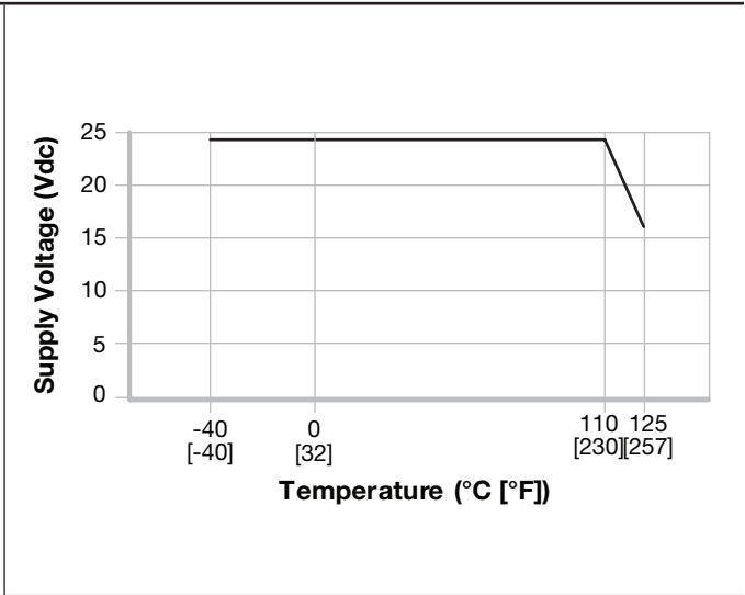
Figure 3. SS360NT, SS360ST, SS360ST-10K Maximum Rated Supply Voltage vs Temperature
