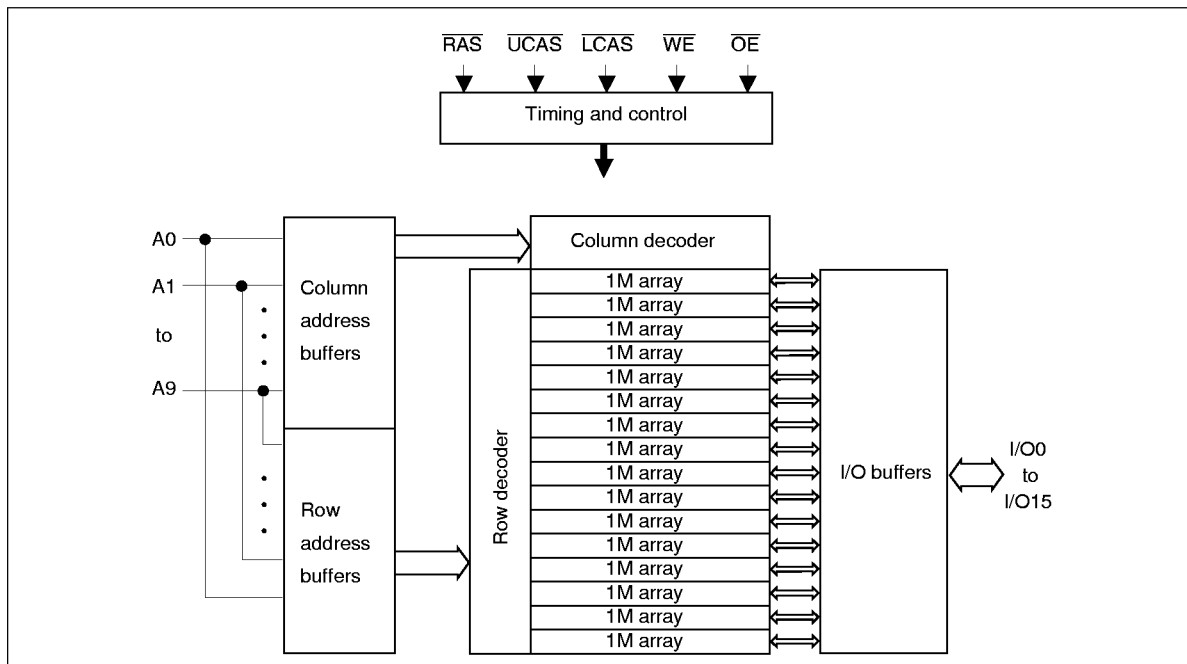
Block Diagram(HM5118160 Series)
