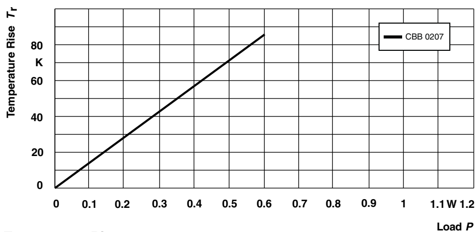
Temperature Rise
