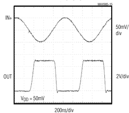
1MHz RESPONSE
