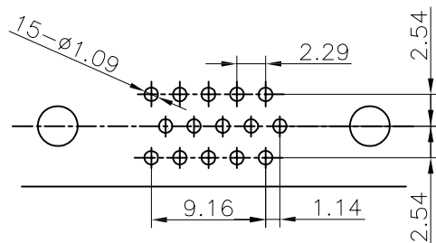
PCB Holes Diagram(Top View)
