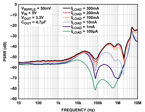
Figure 23. ADP1706 Power Supply Rejection Ratio (PSRR) vs. Frequency
