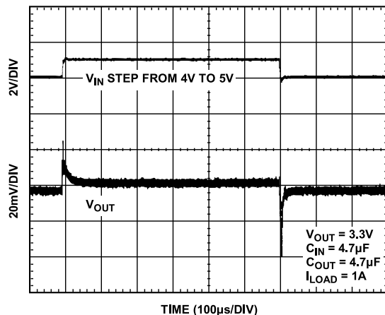
Figure 21. Line Transient Response
