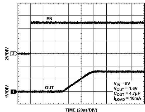
Figure 29. OUT Ramp-Up with Internal Soft Start
