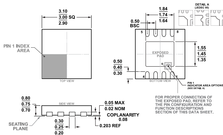
Figure 44. 8-Lead Frame Chip Scale Package [LFCSP] 3 mm x 3 mm Body and 0.75 mm Package Height (CP-8-13)
