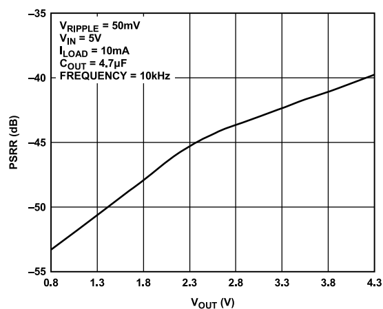
Figure 26. ADP1708 Power Supply Rejection Ratio (PSRR) vs. Output Voltage ( V_{OUT} )
