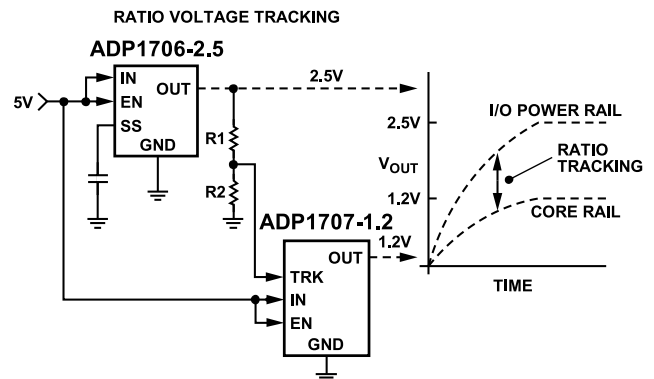
Figure 35. Voltage Tracking Feature Using the ADP1707
