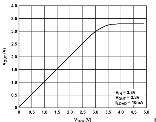
Figure 30. ADP1707 Output Voltage vs. Tracking Voltage
