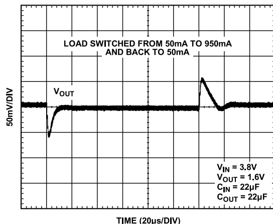
Figure 20. Load Transient Response, C_{\text{IN}} = 22\mu\text{F} , C_{\text{OUT}} = 22\mu\text{F}
