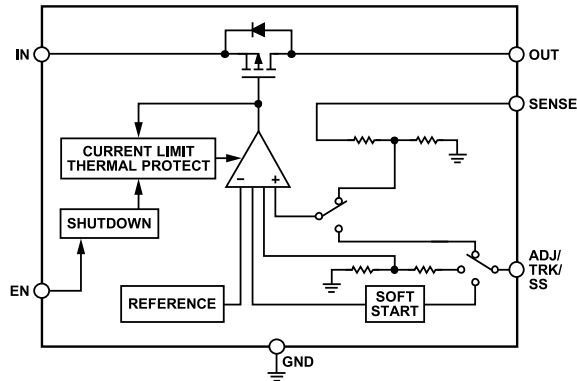
Figure 27. Internal Block Diagram
