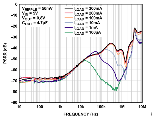
Figure 24. ADP1708 Power Supply Rejection Ratio (PSRR) vs. Frequency
