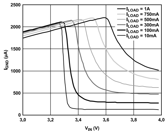
Figure 18. Ground Current ( I_{\text{GND}} ) vs. Input Voltage ( V_{\text{IN}} ) (in Dropout)
