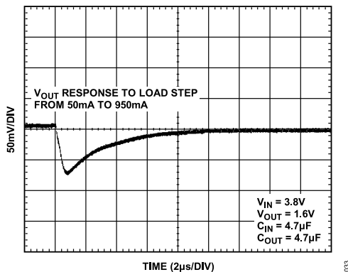
Figure 33. Output Transient Response, C_{OUT} = 4.7 \mu\text{F}
