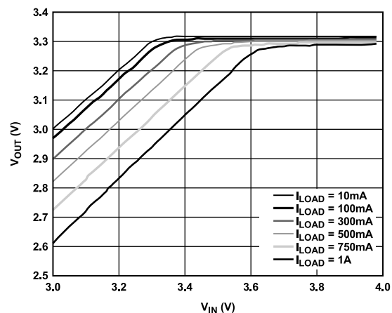
Figure 17. Output Voltage ( V_{\text{OUT}} ) vs. Input Voltage ( V_{\text{IN}} ) (in Dropout)
