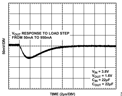
Figure 34. Output Transient Response, C_{OUT} = 22 \mu\text{F}
