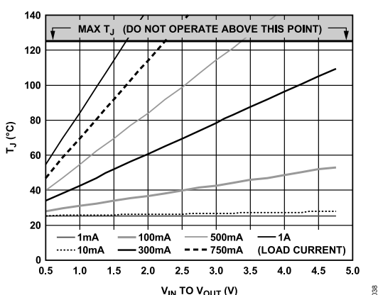
Figure 39. 500 mm 2 of PCB Copper, T_A = 25^\circ\text{C} , LFCSP
