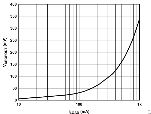
Figure 16. Dropout Voltage ( V_{\text{DROP}} ) vs. Load Current ( I_{\text{LOAD}} )
