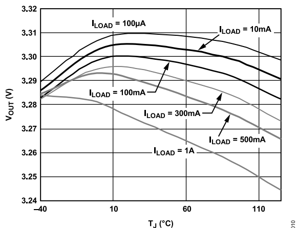
Figure 10. Output Voltage ( V_{OUT} ) vs. Junction Temperature ( T_J )
