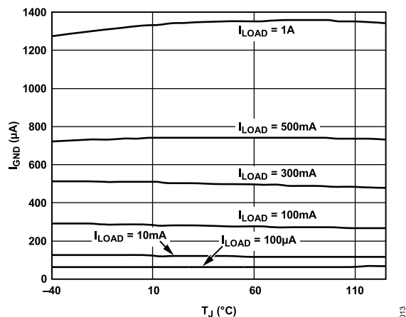
Figure 13. Ground Current ( I_{GND} ) vs. Junction Temperature ( T_J )
