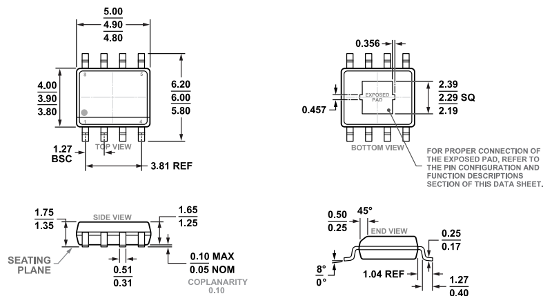
Figure 43. 8-Lead Standard Small Outline Package, with Exposed Pad [SOIC_N_EP] Narrow Body (RD-8-1)
