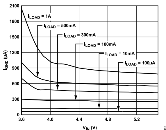
Figure 15. Ground Current ( I_{GND} ) vs. Input Voltage ( V_{IN} )
