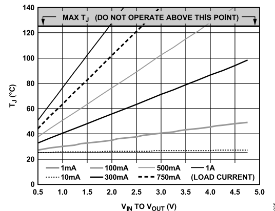
Figure 36. 500 mm 2 of PCB Copper, T_A = 25^\circ\text{C} , SOIC
