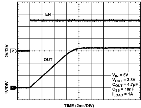
Figure 28. OUT Ramp-Up with External Soft Start Capacitor
