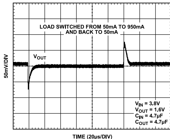
Figure 19. Load Transient Response, C_{\text{IN}} = 4.7\mu\text{F} , C_{\text{OUT}} = 4.7\mu\text{F}
