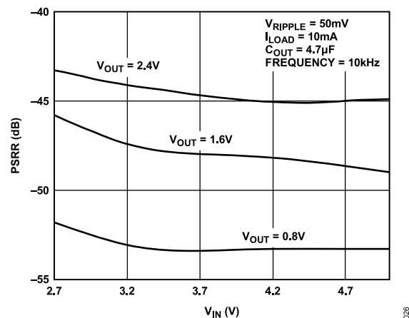
Figure 25. ADP1708 Power Supply Rejection Ratio (PSRR) vs. Input Voltage ( V_{IN} )
