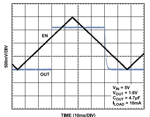
Figure 31. ADP1706 Typical EN Pin Operation
