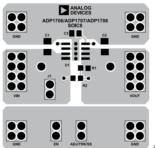
Figure 42. Example PCB Layout
