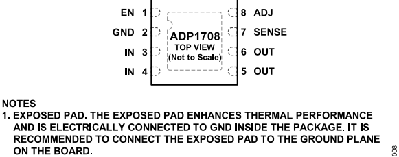
Figure 9. 8-Lead LFCSP, ADP1708
