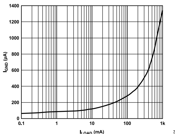
Figure 14. Ground Current ( I_{GND} ) vs. Load Current ( I_{LOAD} )
