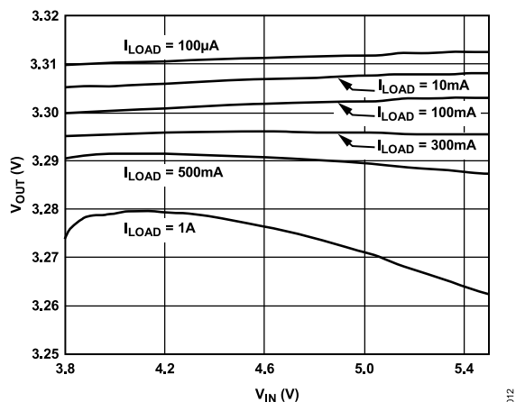
Figure 12. Output Voltage ( V_{OUT} ) vs. Input Voltage ( V_{IN} )
