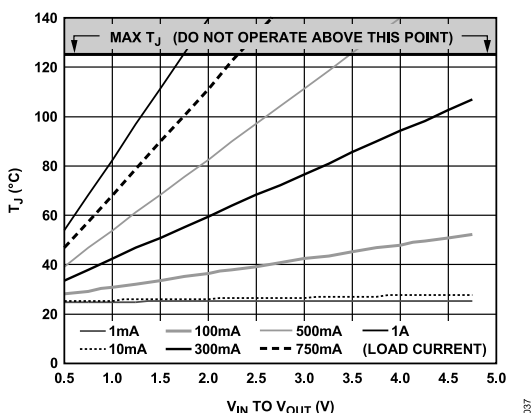
Figure 38. 0 mm 2 of PCB Copper, T_A = 25^\circ\text{C} , SOIC
