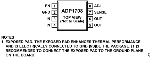
Figure 8. 8-Lead SOIC, ADP1708
