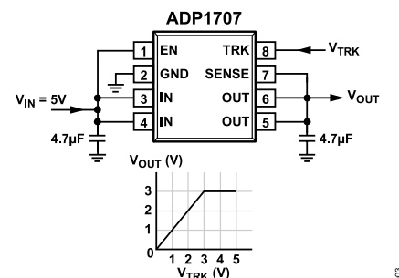
Figure 2. ADP1707 with Output Voltage Tracking
