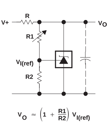
Figure 5. Shunt Regulator
