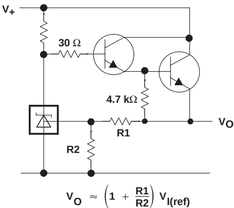
Figure 6. Series Regulator
