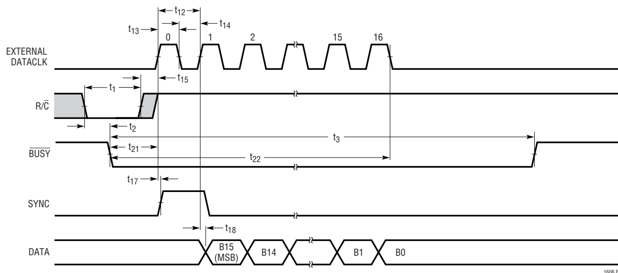
Figure 11. Conversion and Read Timing Using a Discontinuous Data Clock (EXT/INT Tied High, \overline{\text{CS}} Tied Low). Read Previous Conversion Result During the Conversion. For Best Performance, Complete Read in Less Than 1.2 \mu\text{s}
