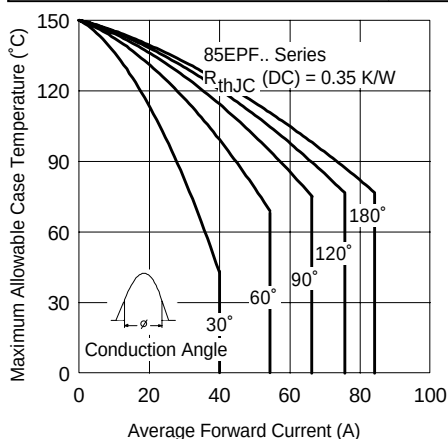
Fig.1-Current Rating Characteristics
