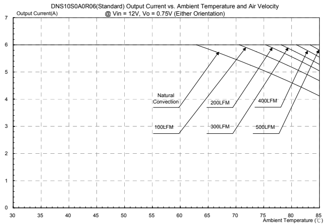
Figure 33: DNS0A0R06(Standard) Output current vs. ambient temperature and air velocity@ Vin=12V, Vout=0.75V (Either Orientation)
