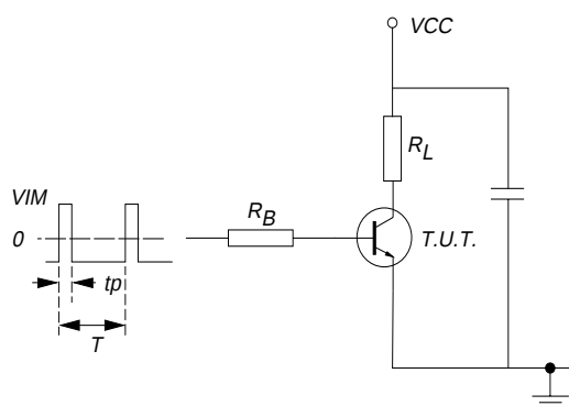
Fig. 11. Test circuit resistive load. V_{IM} = -6 \text{ to } +8 \text{ V} V_{CC} = 250 \text{ V} ; t_p = 20 \mu\text{s} ; \delta = t_p / T = 0.01 . R_B and R_L calculated from I_{Con} and I_{Bon} requirements.
