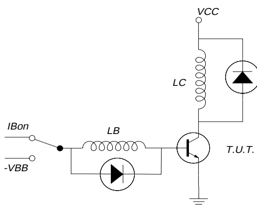
Fig. 9. Test circuit inductive load. V_{CC} = 300 \text{ V} ; -V_{BE} = 5 \text{ V} , L_C = 200 \mu\text{H} ; L_B = 1 \mu\text{H}
