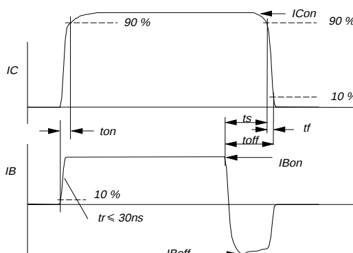
Fig. 12. Switching times waveforms with resistive load.
