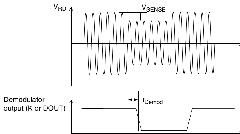
Figure 12 : Demodulator parameters definition
