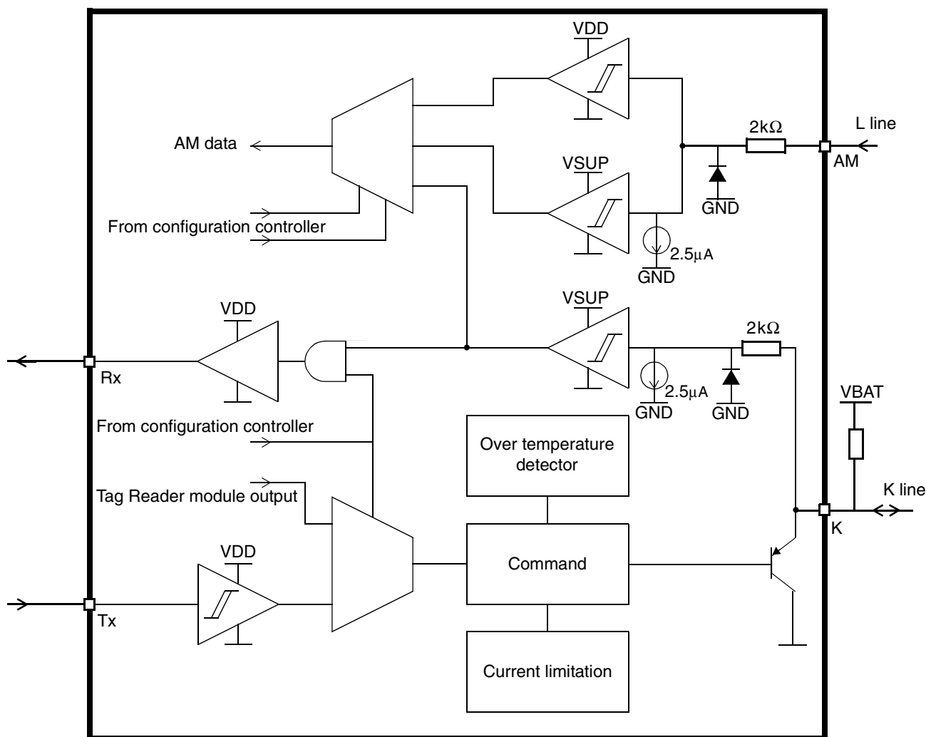
Figure 5 : ISO 9141 interface
