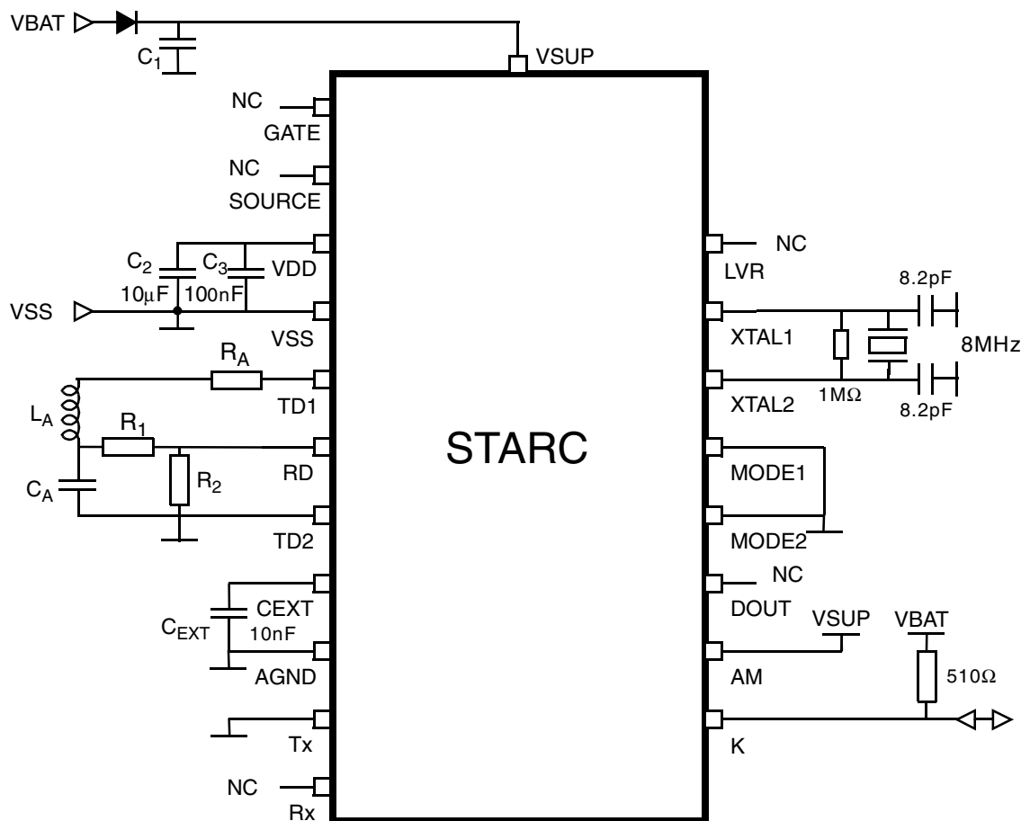
Figure 13 : Standalone configuration with one wire bus
