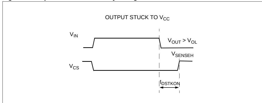
Figure 6. Switching characteristics
