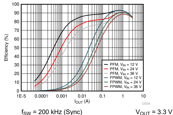
图 7-4. Efficiency vs Load Current
