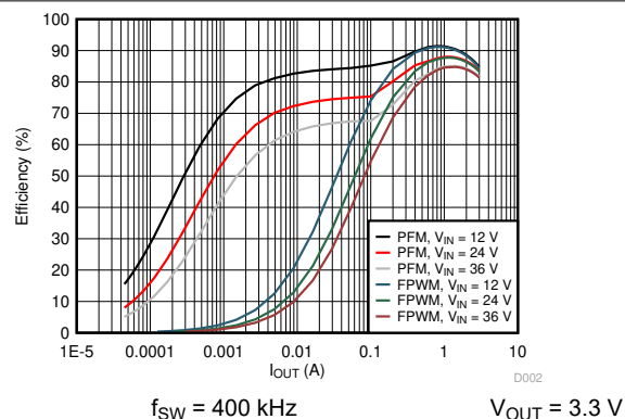
图 7-2. Efficiency vs Load Current
