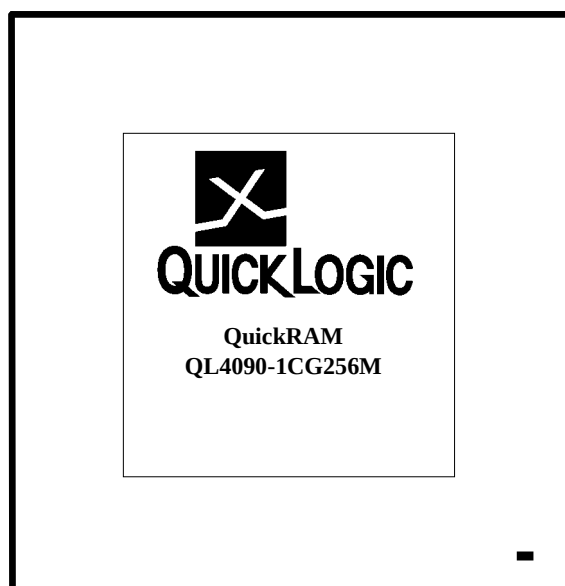
256-Pin CPGA
