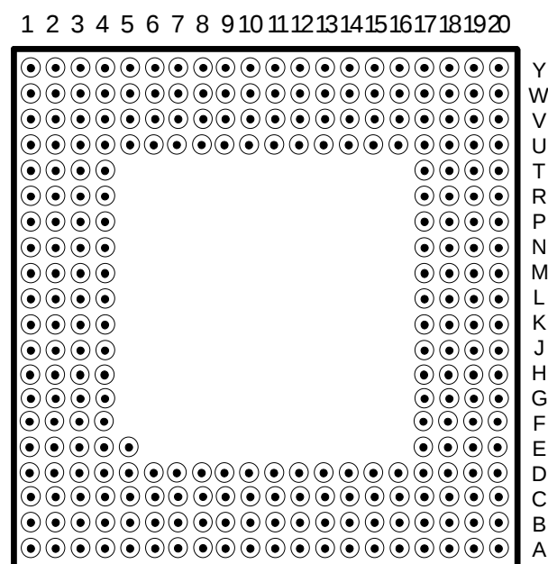
256-Pin CPGA
