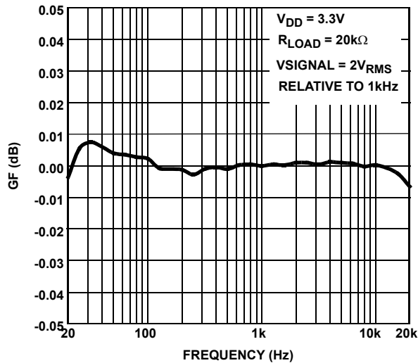
FIGURE 16. GAIN vs FREQUENCY
