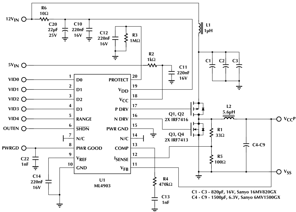
Figure 1. Typical VRM Circuit
