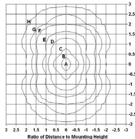
360 Degree Pattern
