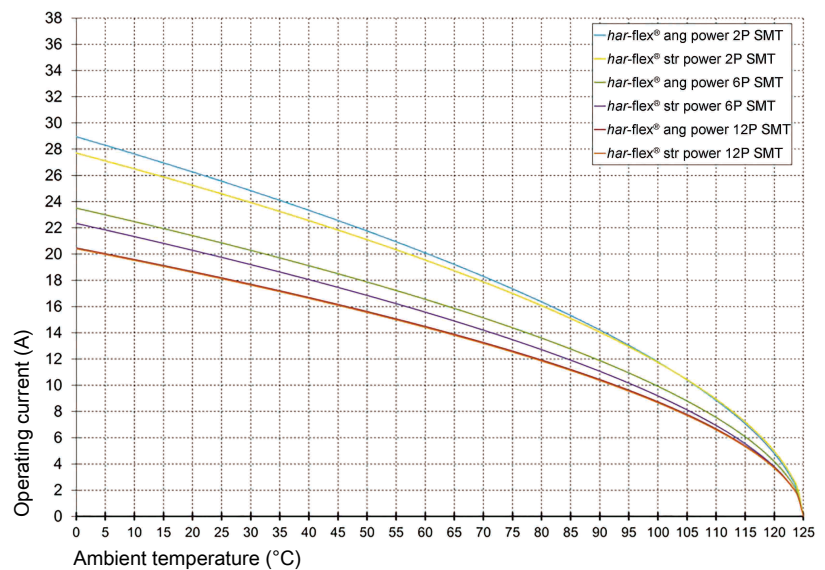
Derating curve 80%
