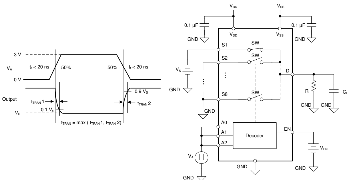
Figure 8-8. Transition Time Measurement Setup
