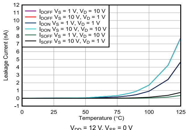
Figure 7-13. Leakage Current vs Temperature
