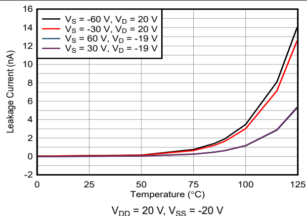
Figure 7-20. I_{D(FA)} Overvoltage Leakage Current vs Temperature
