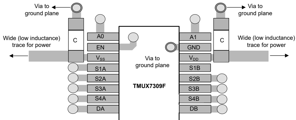
Figure 12-2. TMUX7309FPW Layout Example
