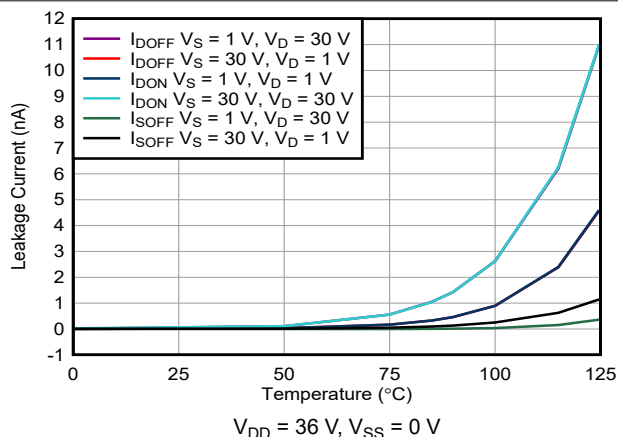
Figure 7-15. Leakage Current vs Temperature
