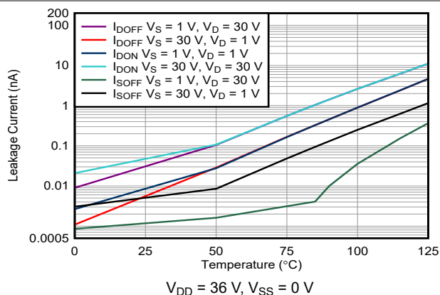
Figure 7-17. Leakage Current vs Temperature
