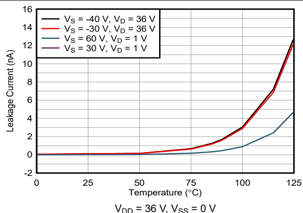
Figure 7-22. I_{D(FA)} Overvoltage Leakage Current vs Temperature
