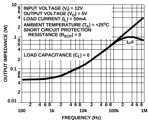
FIGURE 19. OUTPUT IMPEDANCE vs FREQUENCY
