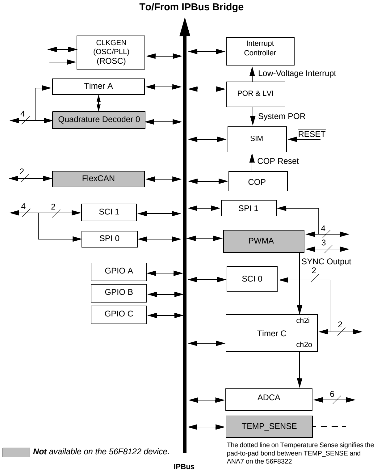
Figure 1-2 Peripheral Subsystem
