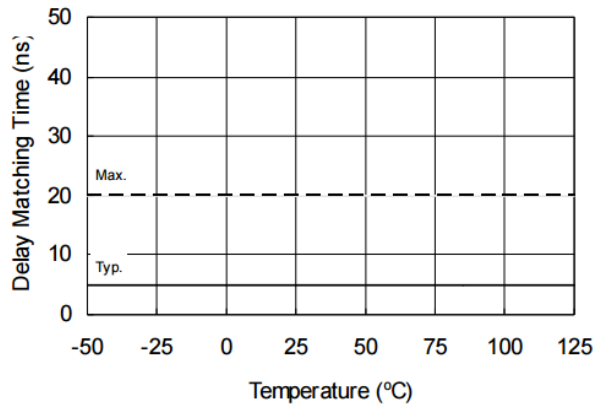
Figure 6A. Turn-on Delay Matching vs. Temperature
