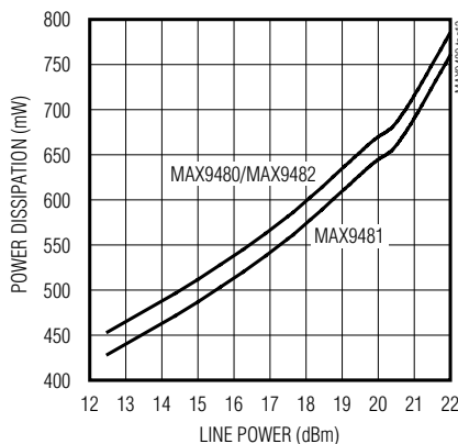
POWER DISSIPATION vs. LINE POWER
