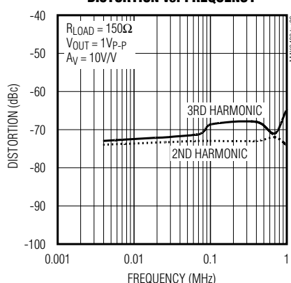
RECEIVER AMPLIFIER HARMONIC DISTORTION vs. FREQUENCY
