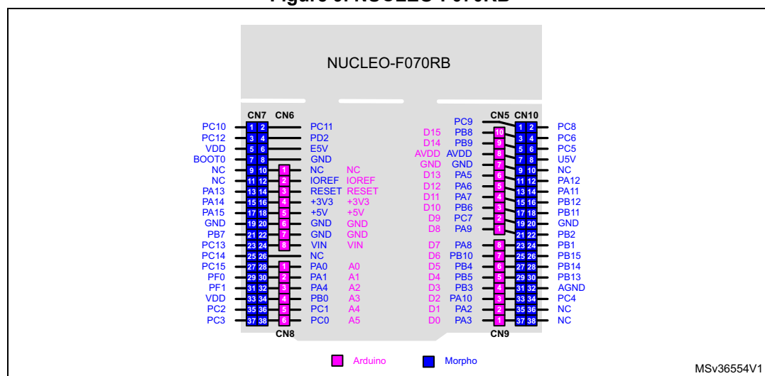
Figure 9. NUCLEO-F070RB
