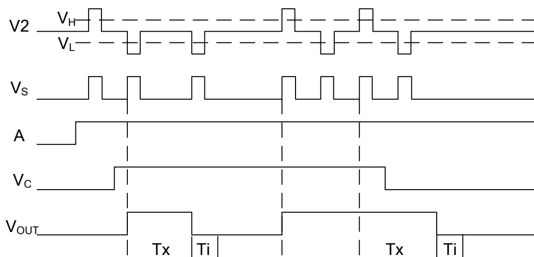
Non-Retriggerable Waveform
