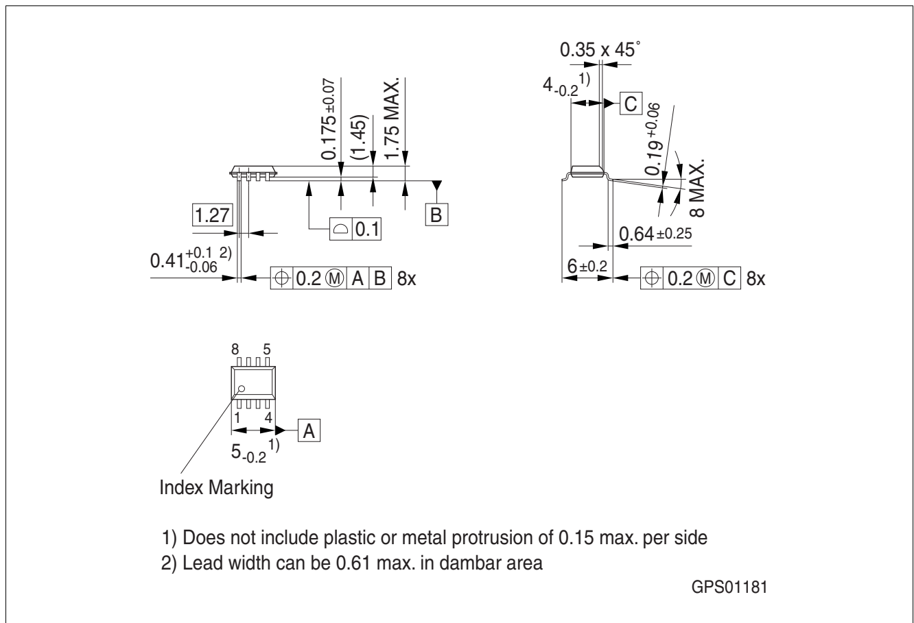
Figure 10 PG-DSO-8
