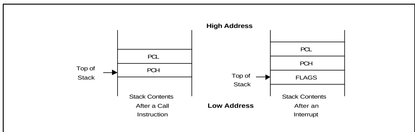
Figure 2-4. Stack Operations
