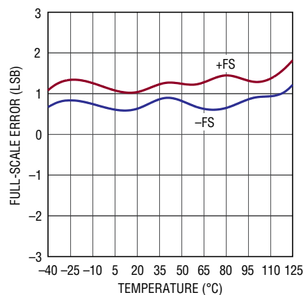
Full-Scale Error vs Temperature REF_{\text{BUF}} = 4.096\text{V}
