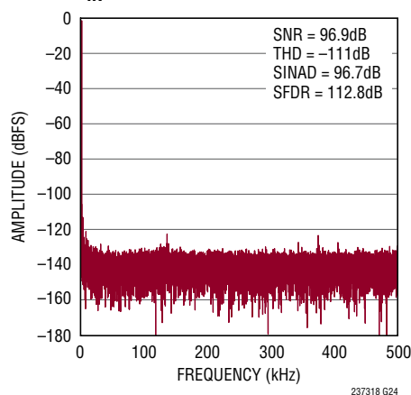
32k Point FFT f_{SAMPL} = 1\text{Mpsps} , f_{IN} = 1\text{kHz} , REF_{BUF} = 5\text{V}
