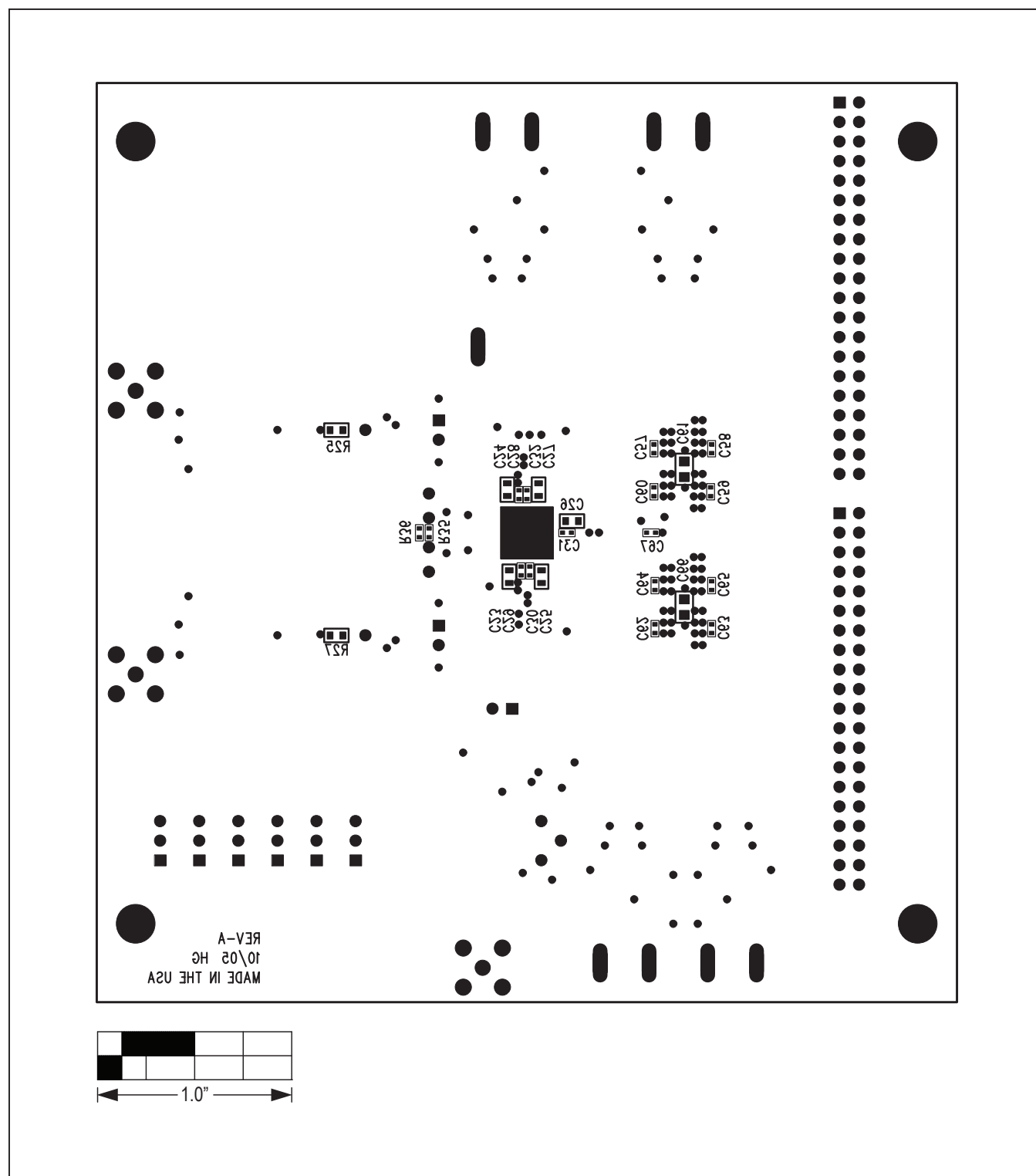
Figure 13. MAX12527/MAX12528/MAX12529/MAX12557/MAX12558/MAX12559 EV Kit PC Board Component Placement Guide—Solder Side
