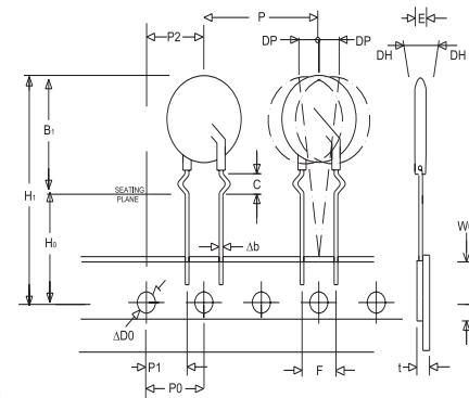
TMOV varistor with outer crimp
