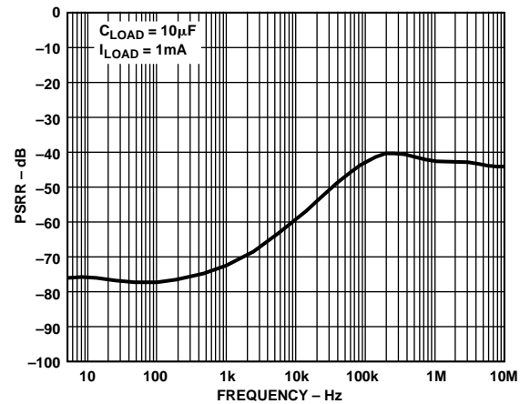
Figure 12. Ripple Rejection*
