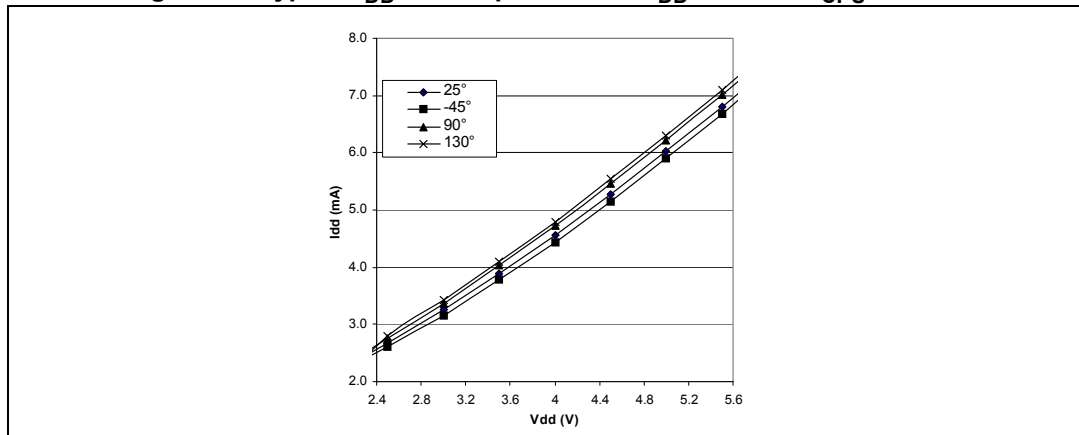
Figure 65. Typical I_{DD} vs. temperature at V_{DD} = 5V and f_{CPU} = 8MHz
