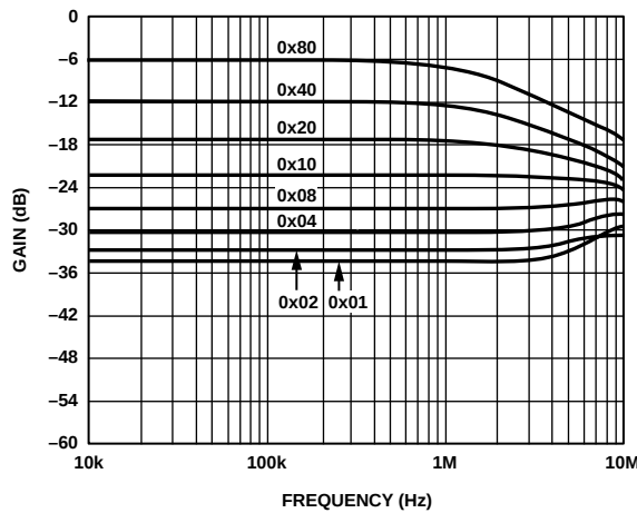
Figure 16. Gain vs. Frequency vs. Code, R_{AB} = 2.5 k\Omega
