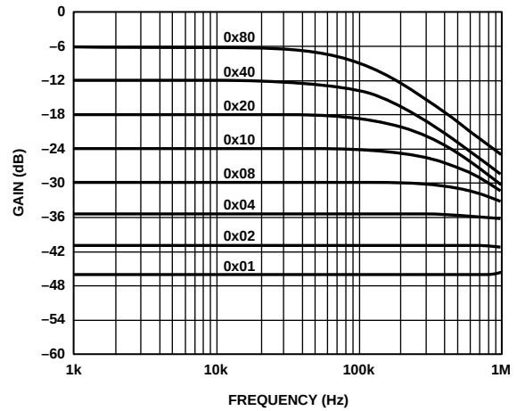
Figure 18. Gain vs. Frequency vs. Code, R_{AB} = 50 k\Omega
