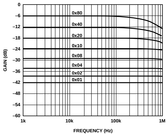
Figure 17. Gain vs. Frequency vs. Code, R_{AB} = 10 k\Omega
