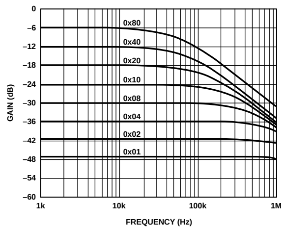
Figure 19. Gain vs. Frequency vs. Code, R_{AB} = 100 k\Omega
