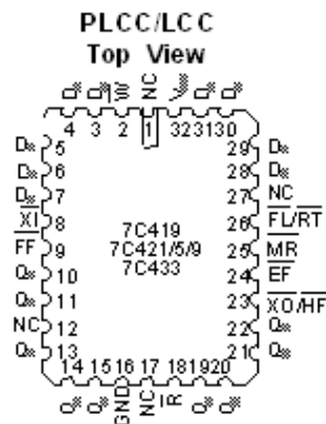
Figure 1. 32-Pin PLCC/LCC
