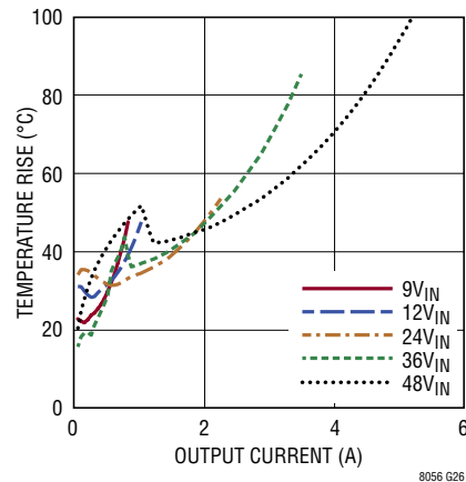
Temperature Rise vs Output Current ( 36V_{OUT} )
