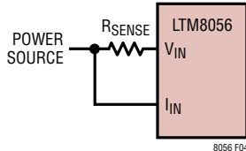
Figure 4. Set the LTM8056 Input Current Limit with an External Sense Resistor
