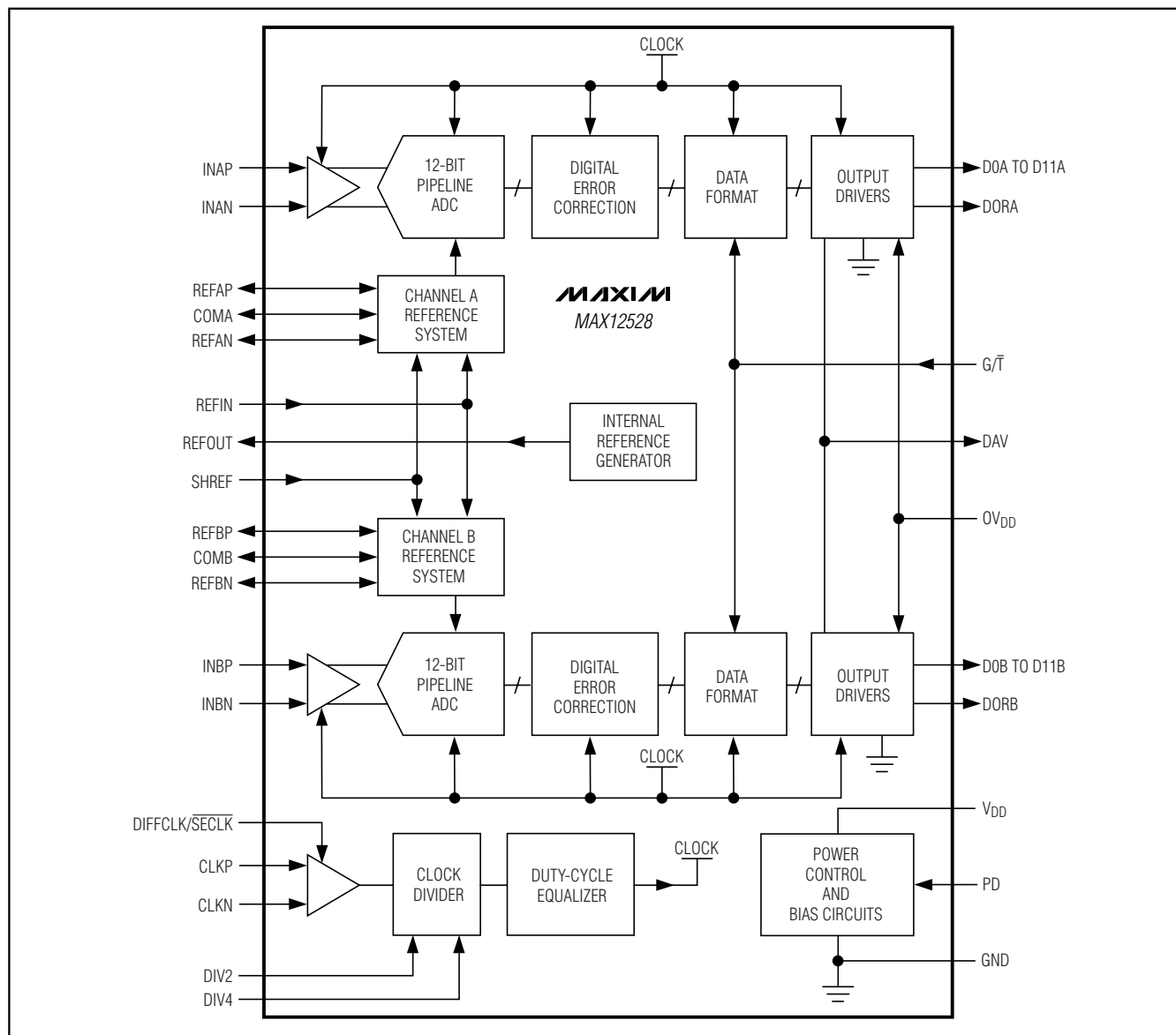
Figure 2. Functional Diagram
