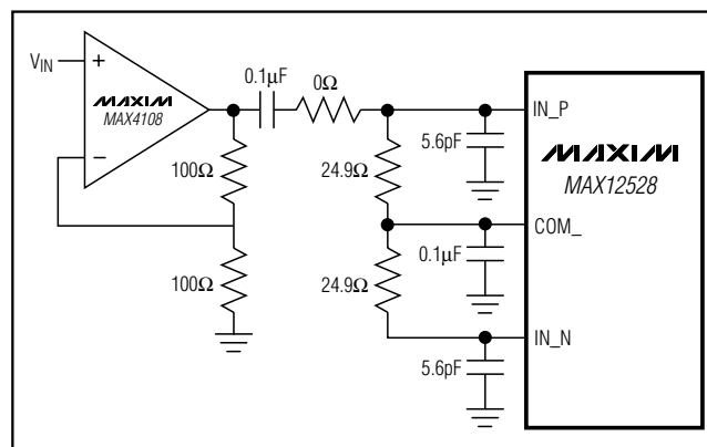
Figure 11. Single-Ended, AC-Coupled Input Drive
