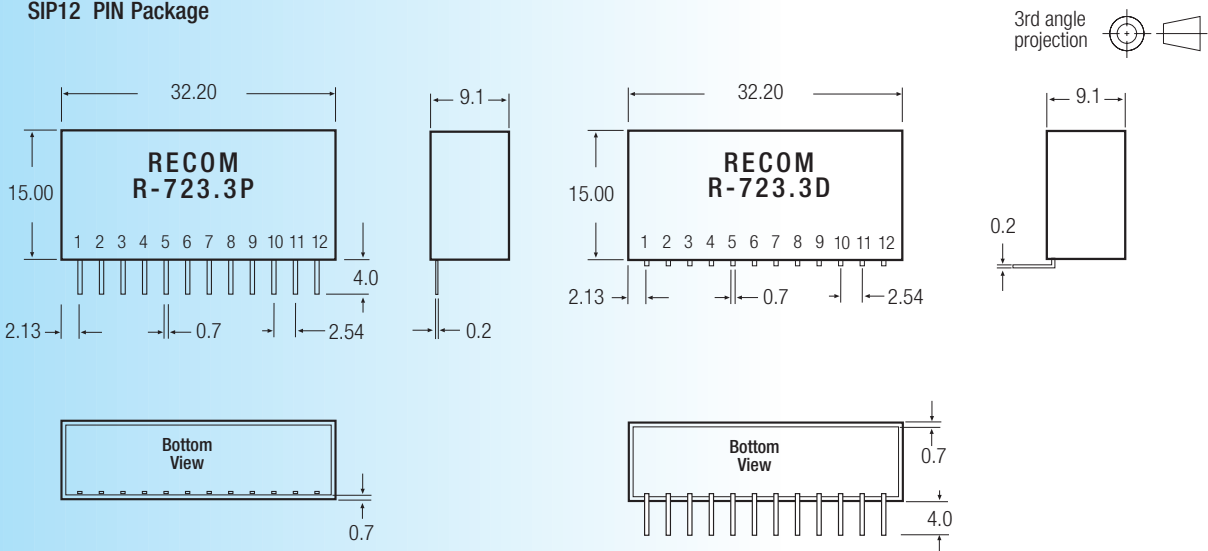
SIP12 PIN Package
