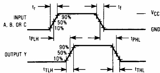
Figure 1. Switching Waveforms
