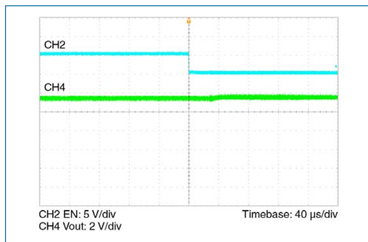
Figure 18 — Three module parallel array test. Vout change with two modules operating and a third module enabled. Nominal
