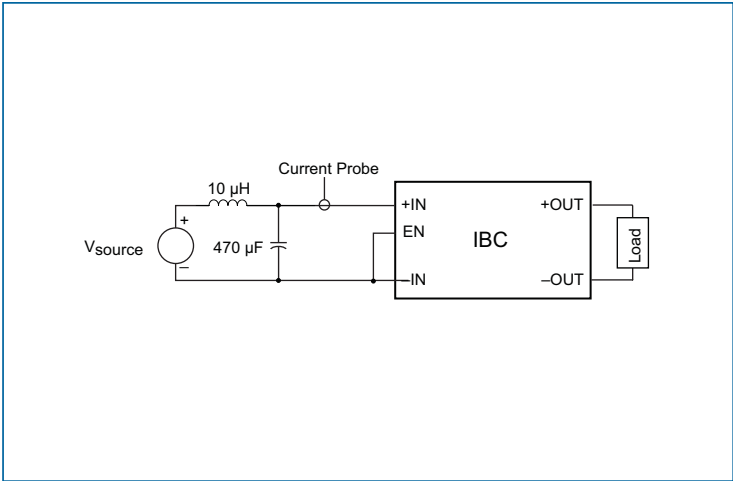
Figure 22 — Test circuit; input reflected ripple current
