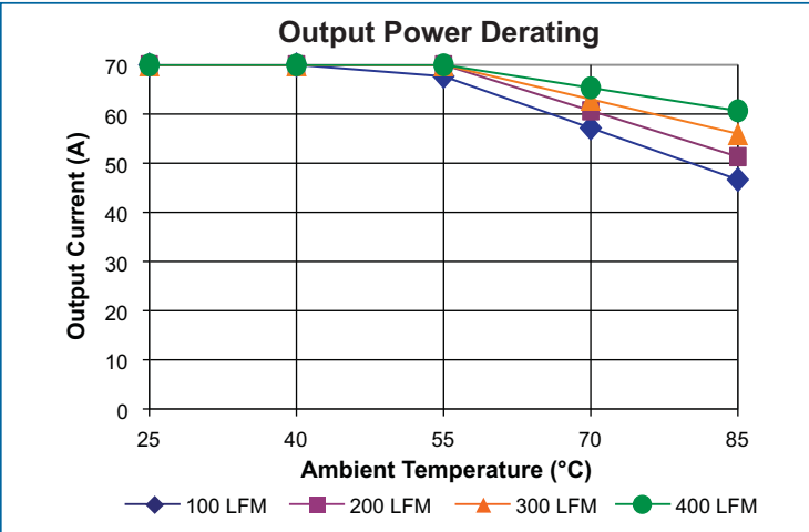
Figure 19 — Maximum output power derating vs ambient air temperature. Transverse airflow, Board and junction temperatures <125° C. Tested with IBC evaluation board IB050Q096T70N1-CB
