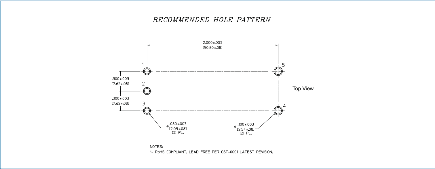
Figure 33 — IBC PCB recommended hole pattern
