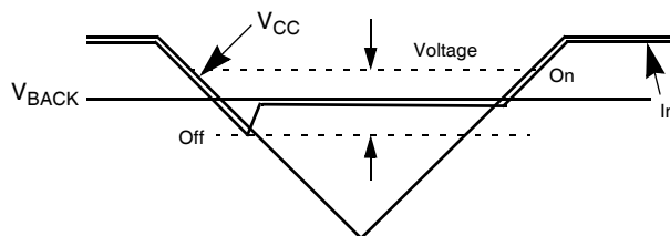
Figure 3. Power Control
