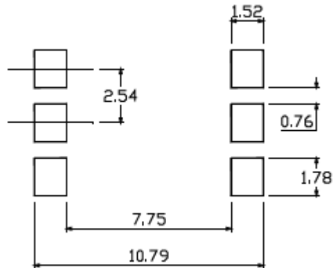
Recommended Solder Footprint for SMD Leadform
