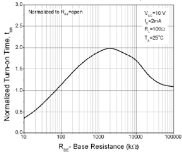
Figure 9. Turn-on Time vs Base-Emitter Resistance
