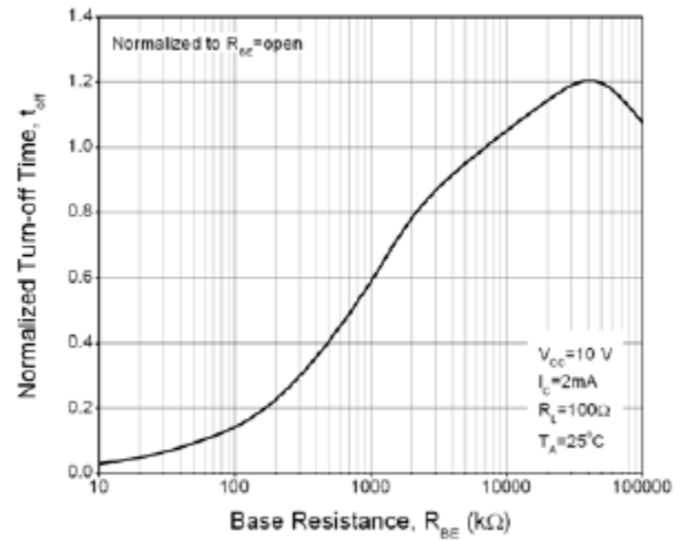
Figure 10. Turn-off Time vs Base-Emitter Resistance
