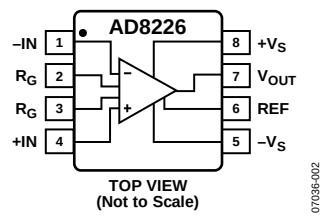
Figure 2. Pin Configuration
