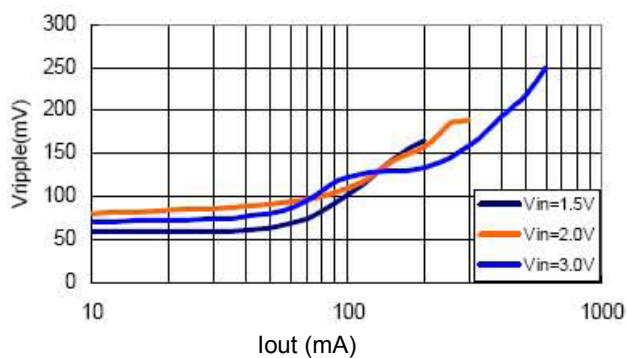
ACE705260BN+ Ripple VS. Output Current
