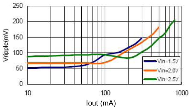
ACE705230BN+ Ripple VS. Output Current
