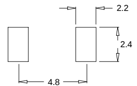
Recommended Pad Layout
