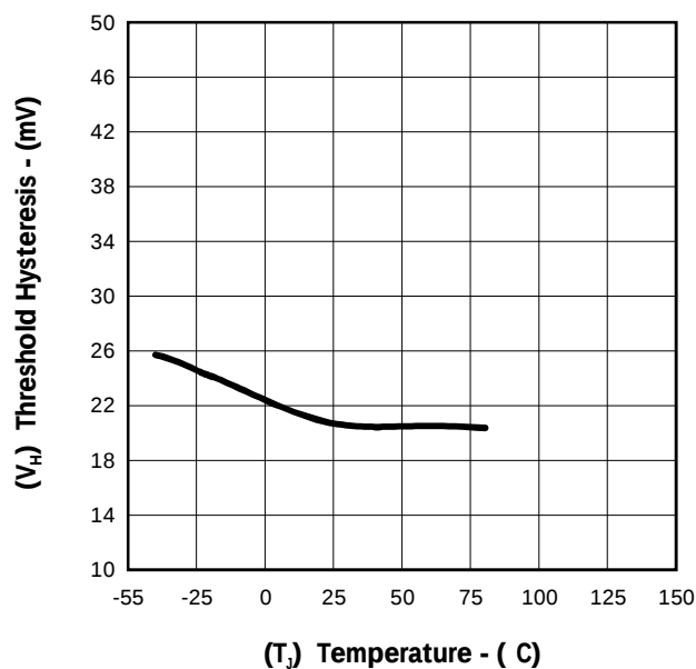
FIGURE 6. — THRESHOLD HYSTERESIS vs. TEMPERATURE
