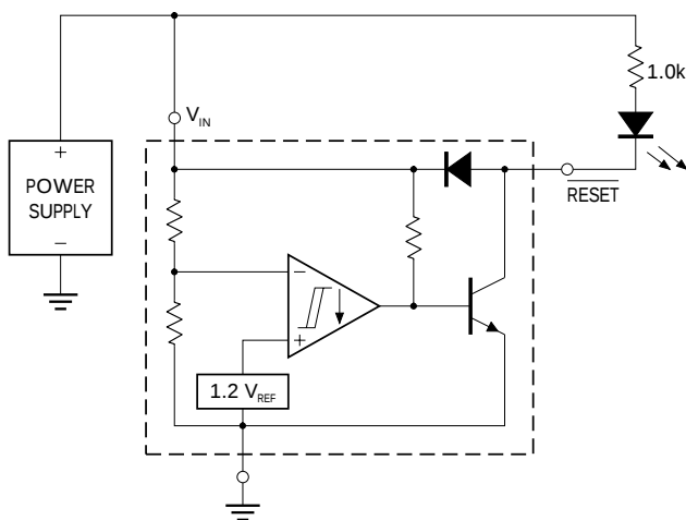
FIGURE 17. — VOLTAGE MONITOR
