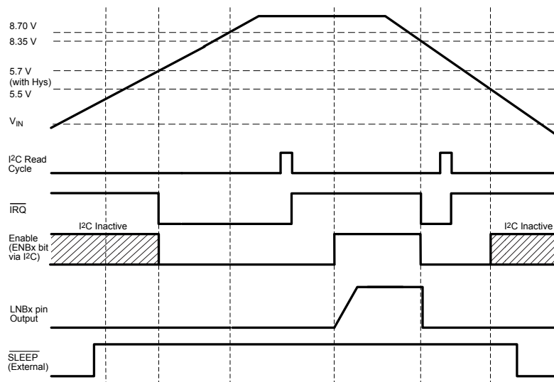
Figure 14b. \overline{IRQ} is cleared when V_{IN} is already above V_{IN(th)} . As the ENBx bit is already set high, LNBx starts rising immediately after an I2C Read sequence.
