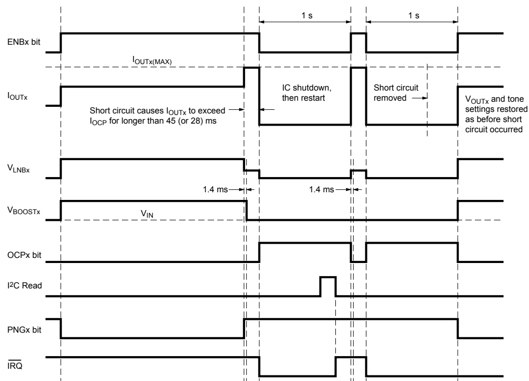
Figure 2a. \overline{\text{IRQ}} and Fault Clearing in Response to Overcurrent (OCP) with auto-retry enabled (RSMODE = 1) and an OCP delay of 45 (or 28) ms (TDIS_T = 1 (or 0)). \overline{\text{IRQ}} transitions to low at an OCP fault and is reset by an I 2 C Read sequence. The OCP bit clears automatically after 1 s, and the device restarts with the previous settings. This hiccup mode continues as long as the output current is greater than the OCP level. The device returns to normal operation when the fault is removed.
