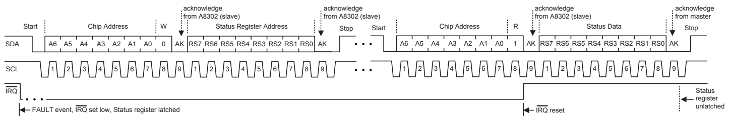
Figure 12. I 2 C™ Interface Read from Status register sequence. The \overline{\text{IRQ}} pin is reset to high when the A8302 acknowledges it is being read. The Status register is unlatched when the master acknowledges the status data from the A8302.
