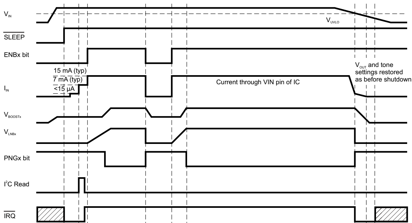
Figure 13. Startup and Shutdown Cases. \overline{IRQ} and Fault Clearing in Response to Undervoltage at VIN (UVLO). If \overline{IRQ} transitions low because of a latched fault, the LNBx output does not respond to the ENBx bit. An I 2 C™ Read sequence is required to clear any latched fault and reset the \overline{IRQ} to logic high. An I 2 C™ Read is required after a UVLO fault.
