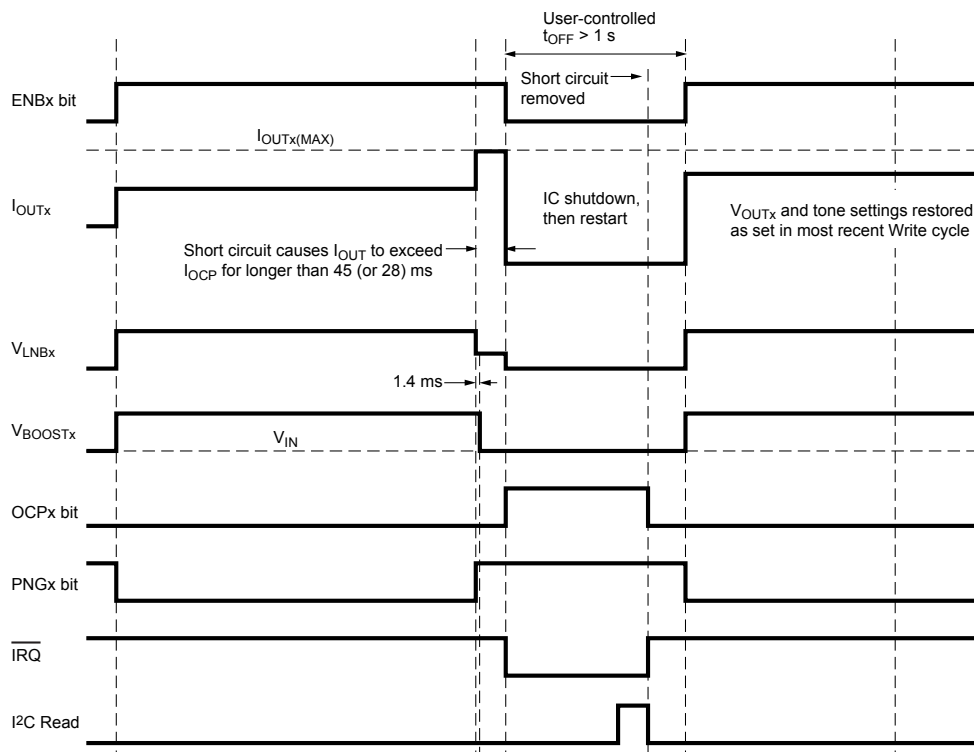
Figure 2b. \overline{\text{IRQ}} and Fault Clearing in Response to Overcurrent (OCP) with latch mode (RSMODE = 0) and an OCP delay of 45 (or 28) ms (TDIS_T = 1(or 0)). \overline{\text{IRQ}} transitions low at an overcurrent fault, and an I 2 C Read sequence clears the OCP bit and \overline{\text{IRQ}} . An I 2 C Write sequence is required to reenables the part. The retry wait time should be longer than 1 s, to prevent TSD.
