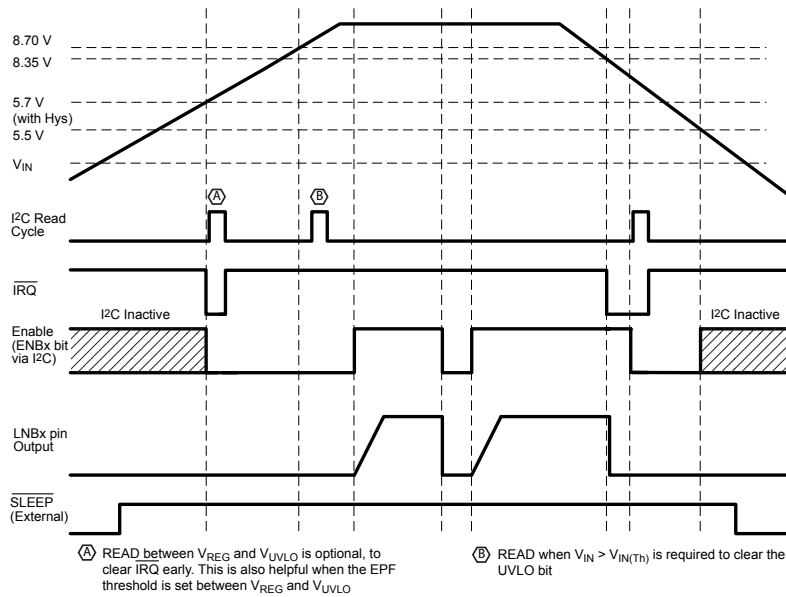
Figure 14a. I2C and \overline{IRQ} operate down to V_{IN} > V_{REG} ( V_{REG} is 5.25 V typical), LNBx and BOOSTx operate from V_{IN(th)} . When V_{IN} exceeds V_{REG} (5.25 V typical), \overline{IRQ} transitions low because of the UVLO fault, and an I2C Read sequence will clear the \overline{IRQ} fault. While powering down, when V_{IN} falls below V_{UVLO} , \overline{IRQ} becomes low, LNBx and BOOSTx turn off, and I2C becomes inactive when V_{IN} falls below V_{REG} .
