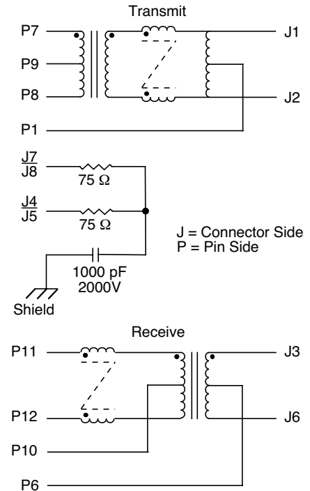
Schematic
