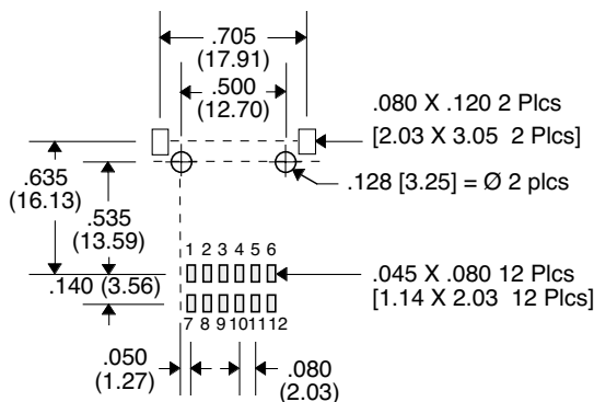
PCB Layout (Component)
