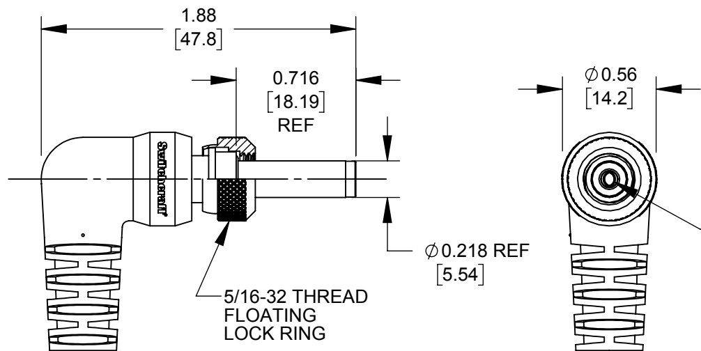
S10KS SERIES SEALED HI-AMP PLUG
