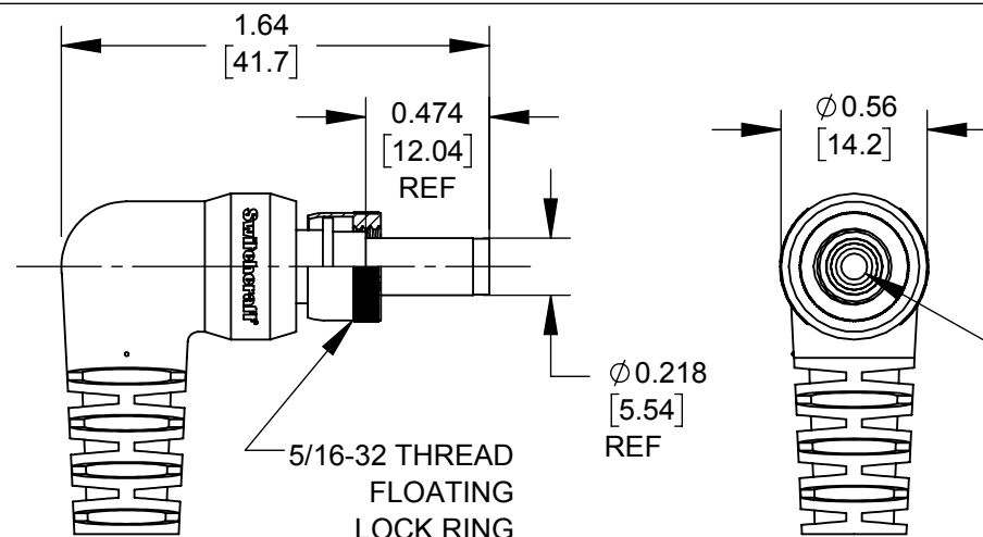
761K, 767K, AND S761K SERIES LOCKING POWER PLUGS
