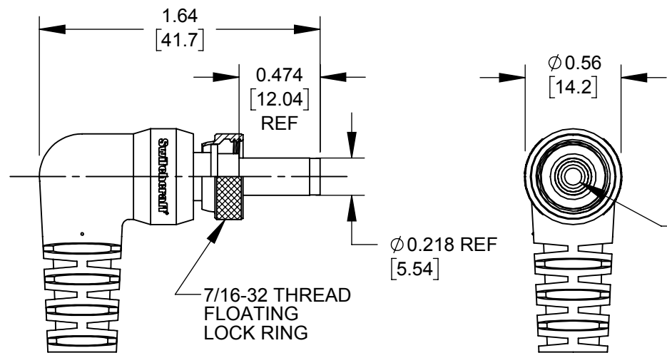
761KS, 767KS, AND S761KS SERIES SEALED PLUGS
