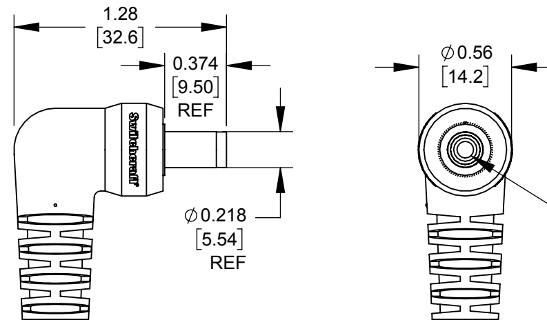
760, 762, AND S760 SERIES NON-LOCKING POWER PLUGS
