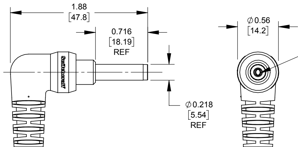
S10 SERIES NON-SEALED NON-LOCKING HI-AMP PLUG
