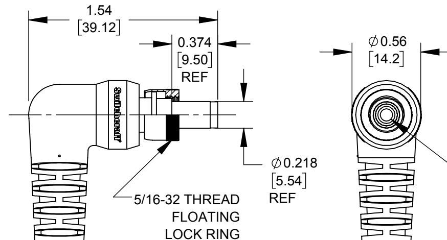
760K, 762K, AND S760K SERIES LOCKING POWER PLUG
