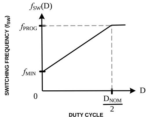
FIGURE 17. ADAPTIVE FREQUENCY
