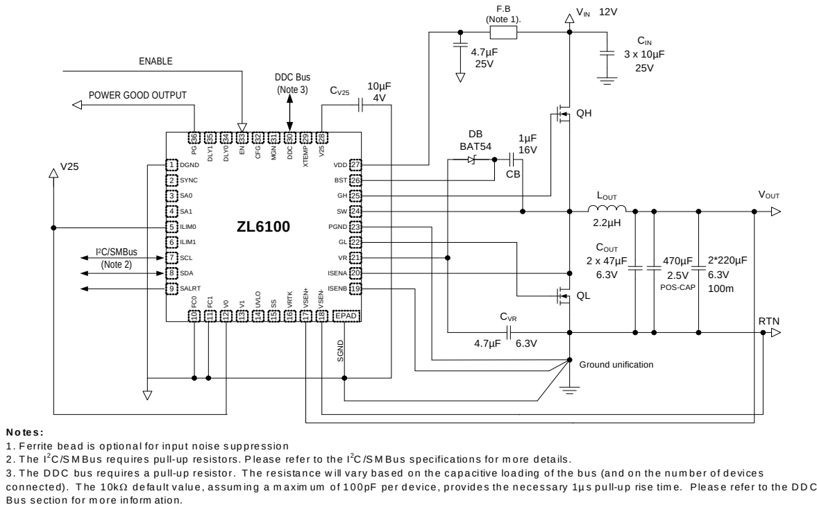
FIGURE 2. 12V TO 1.8V/20A APPLICATION CIRCUIT (4.5V UVLO, 10ms SS DELAY, 5ms SS RAMP)
